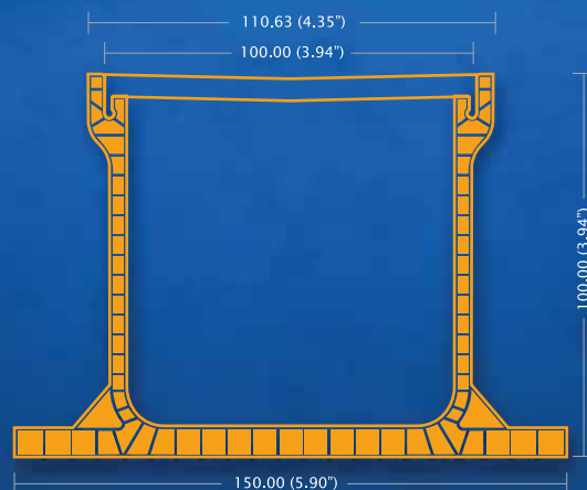
ULTRA DRAIN (100 X 100) Open end discharge 0.5M fall (825L/M)
