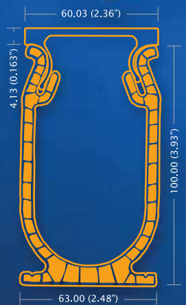
ULTRA DRAIN (60 X 100) Open end discharge 0.5M fall (500 L/M)
