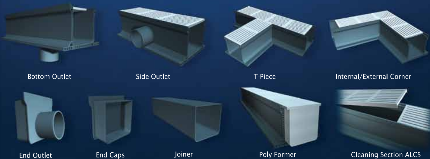
ULTRA DRAIN (60 X 100) Open end discharge 0.5M fall (500 L/M)
