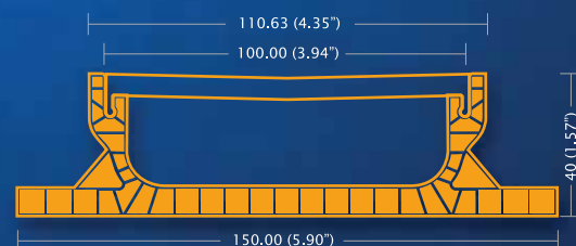
ULTRA DRAIN (40 X 100) Open end discharge 0.5M fall (295L/M)
